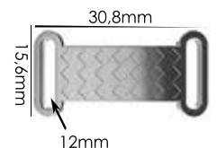
Ref.: AMP 049 12mm
